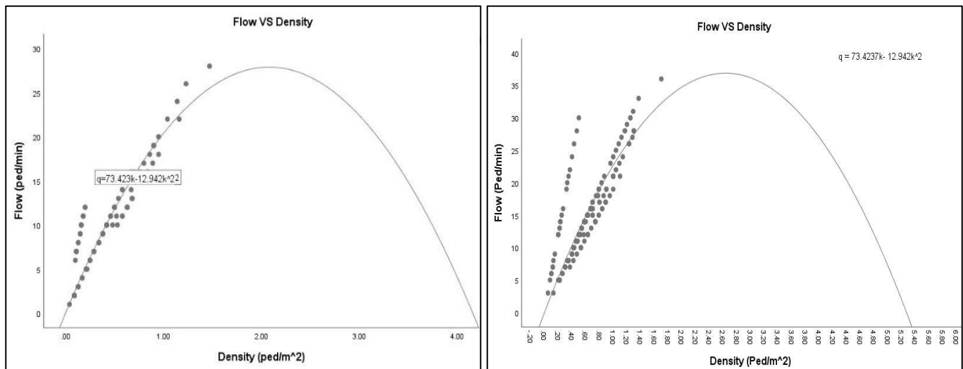
Figure 2: Flow vs Density relationship for walkways at peak (left) and off-peak hour (right)
