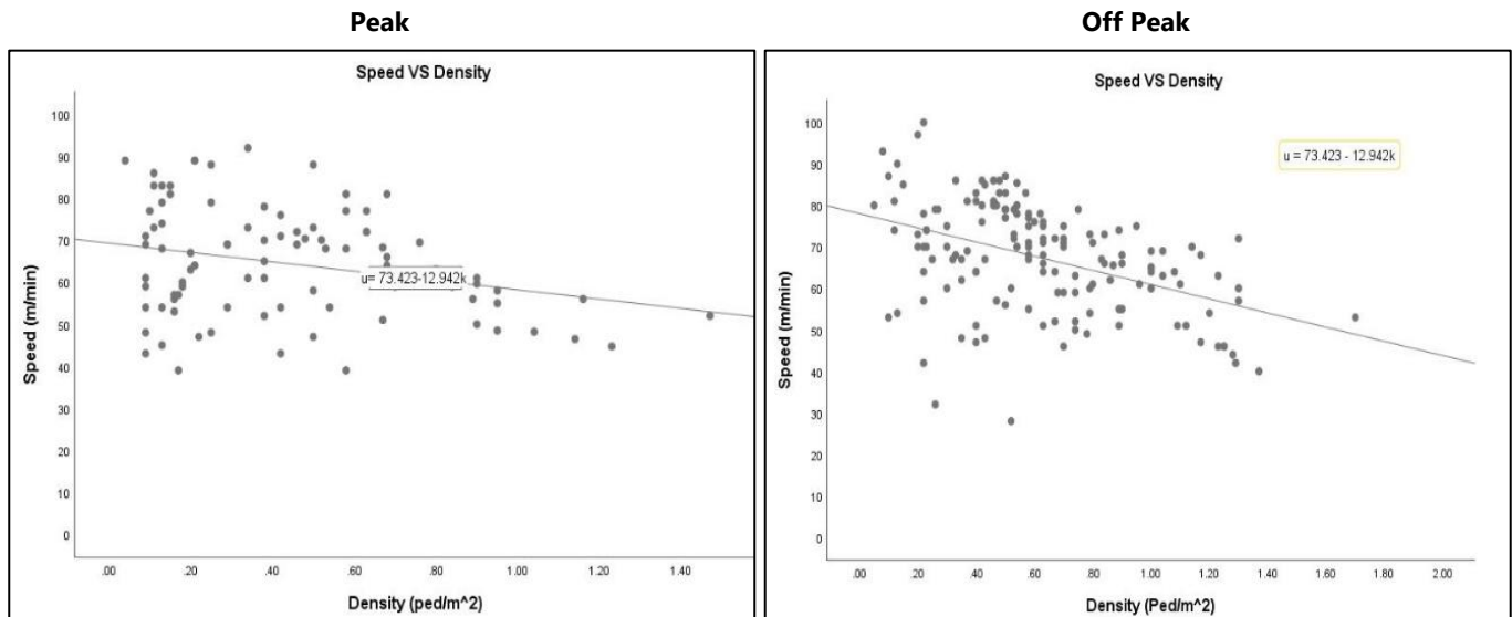
Figure 1: Speed vs Density relationship for walkways at peak (left) and off-peak hour (right)
