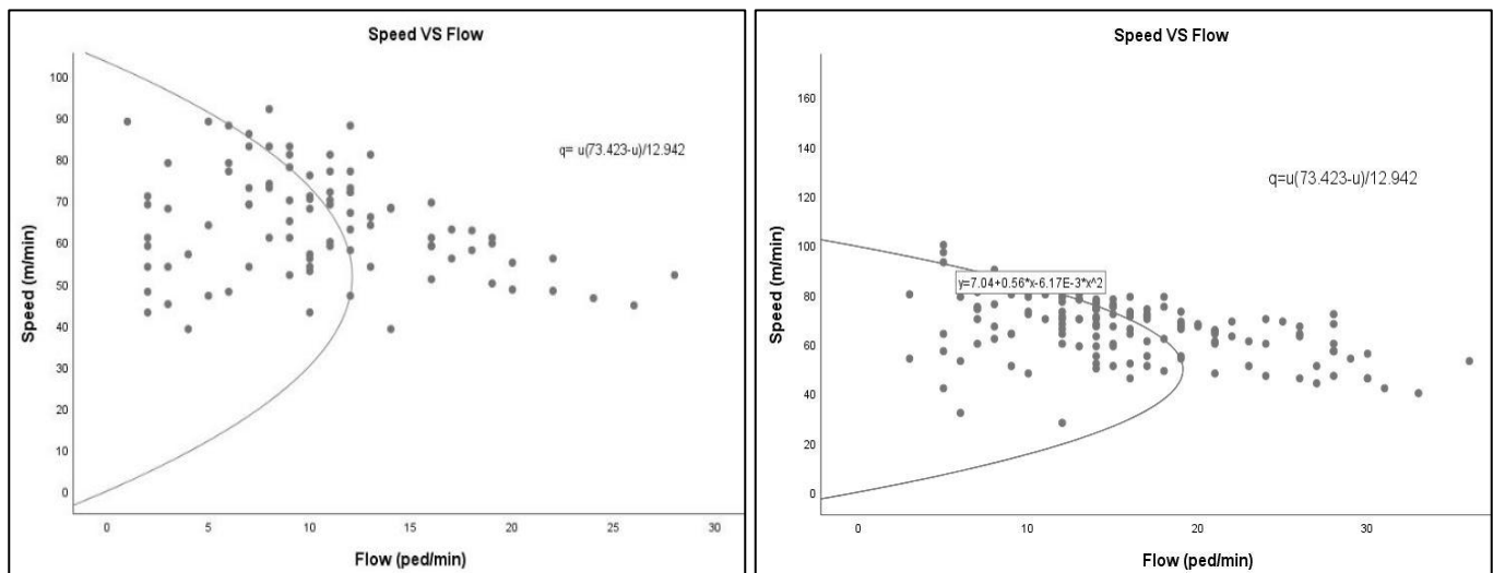
Figure 3: Speed vs Flow relationship for walkways at peak (left) and off-peak hour (right)
