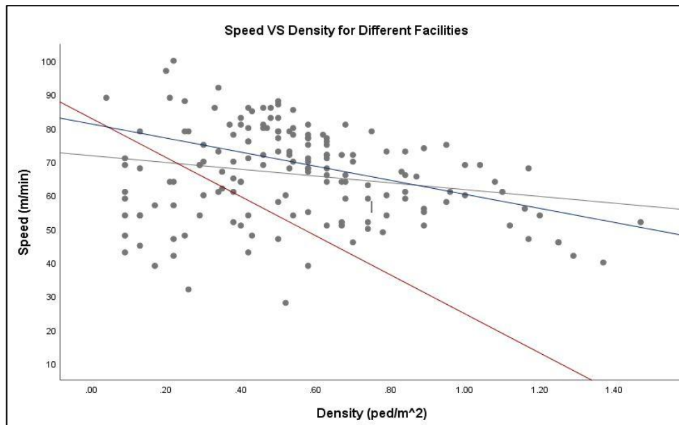
Figure 5: Speed vs density relationship for different pedestrian facilities
