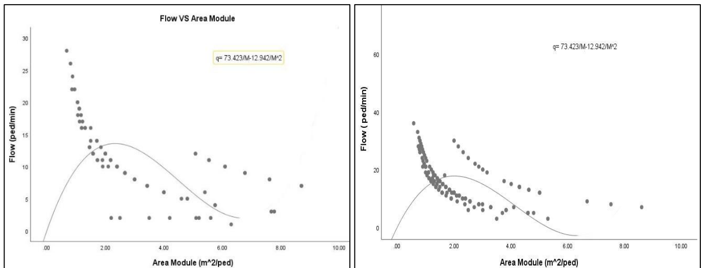
Figure 4: Flow vs Area relationship for walkways at peak (left) and off-peak hour (right)
