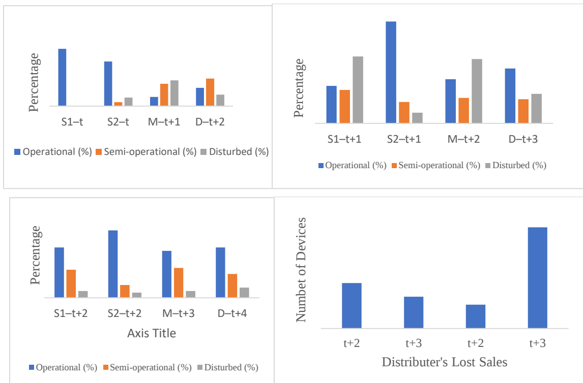
Fig 10. Modeling the ripple effect of complete disruption of both suppliers at time t (Scenario 3).
