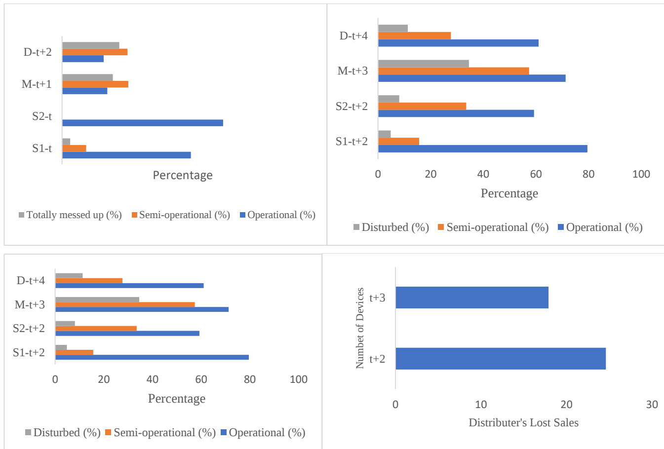
Fig 8. Modeling the ripple effect of complete disruption of the second supplier at time t (Scenario 1).
