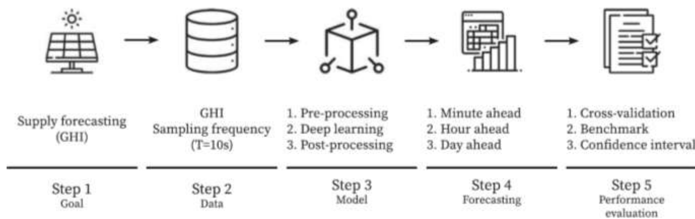
Figure 06: Proposed Supply Forecasting Framework [16]
