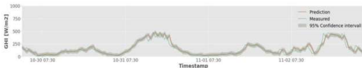
Figure 14: Minutes ahead Global Horizontal Irradiance (GHI) forecast (15 min ahead)
