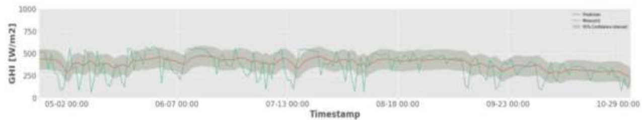
Figure 16: Hours ahead Global Horizontal Irradiance (GHI) forecast (6h ahead)
