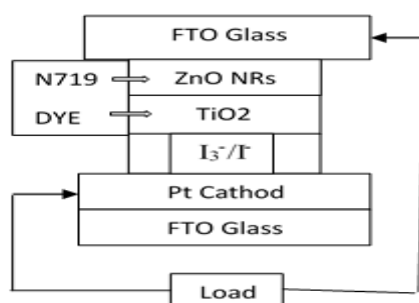
Fig 1. The structure of Dye synthesized solar cell
