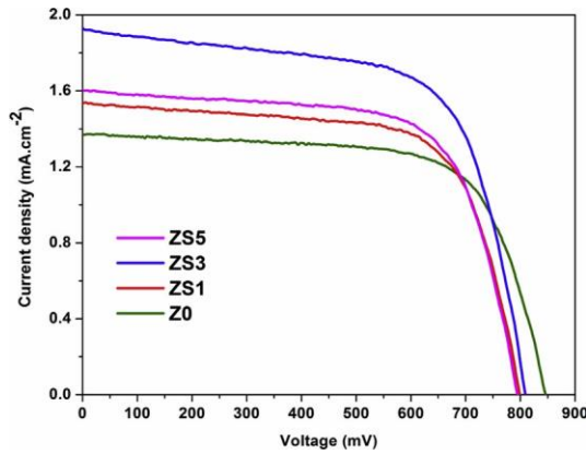
Figure 8. J-V curve of fabricated DSSC using ZnO and Sr doped ZnO based photoanodes Reproduced from (Rajan & Cindrella, 2019) with permission, copyright@2019, Elsevier
