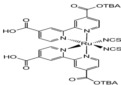
Figure 3. Structure of the N719 dye.
