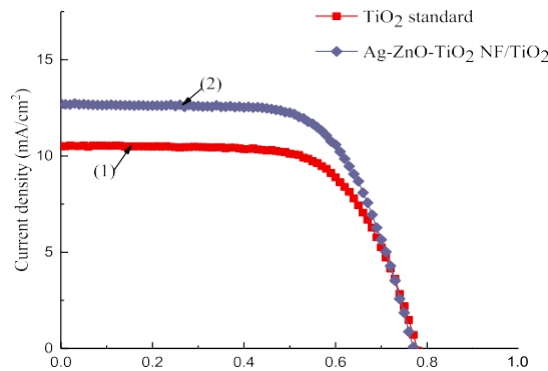
Figure 7. J-V curves of TiO 2 standard DSSC and DSSC modified with Ag-ZnO-TiO 2 NFs. Reproduced from (Nien et al., 2020) with permission, copyright@2020, IEEE
