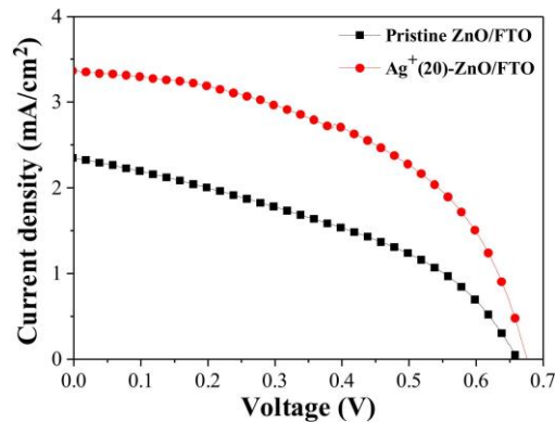
Figure 9. J-V curve of the DSCs with the pristine ZnO/FTO and Ag + (20) ZnO/FTO photo-electrodes, measured under AM 1.5 condition. Reproduced from (Cho et al., 2022) with permission, copyright@2022, MDPI
